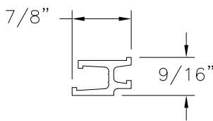
LOCK RAIL/STILE REINFORCEMENT (10712) ALUMINUM 6005-T5
