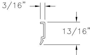
GLAZING BEAD EXTRUDED RIGID PVC
