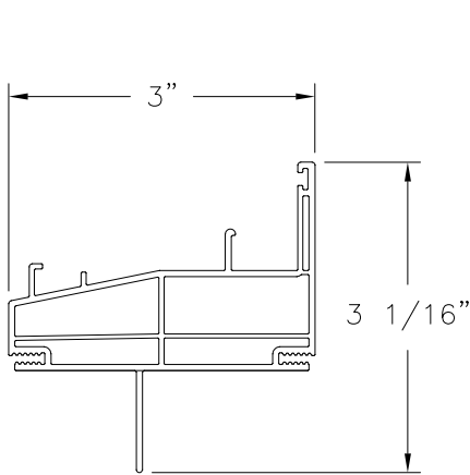
SILL (9202A) EXTRUDED RIGID PVC
