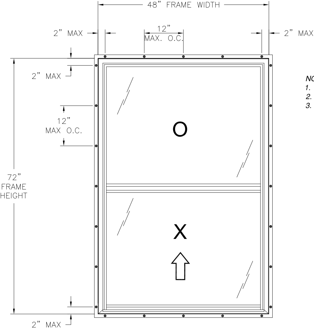
200/275 VINYL SINGLE HUNG WINDOW EXTERIOR VIEW
